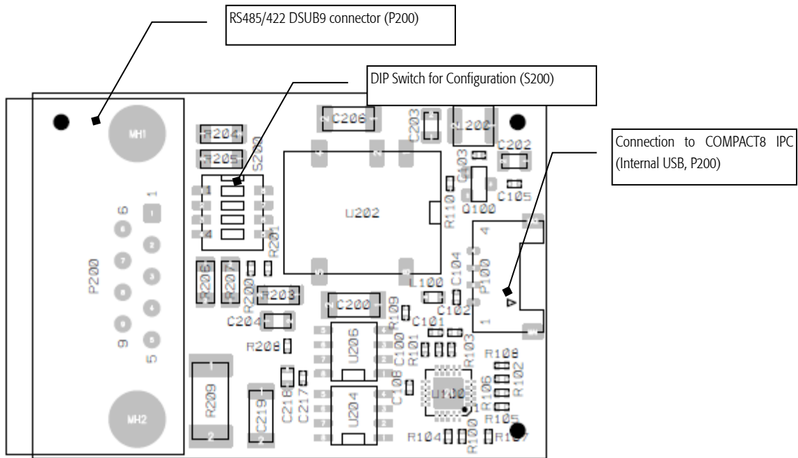
Fig. 3 Board Layout
