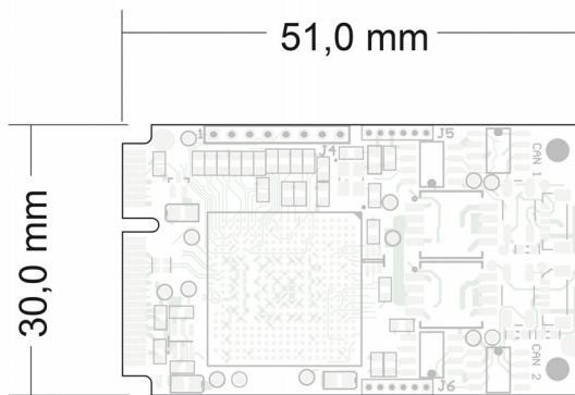
Figure 22: View onto the PCAN-miniPCIE FD Single and Dual Channel (IPEH-004045/46)
