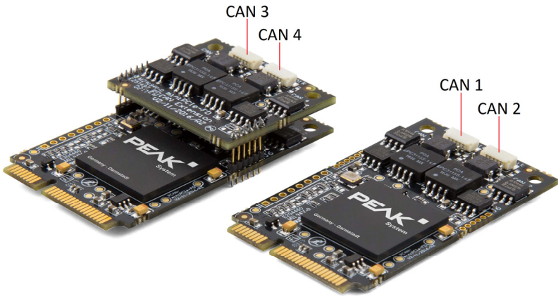
Figure 1: Positions of the CAN ports on the PCAN-miniPCIE FD card; left four-channel and right two-channel card; for the single channel card only CAN 1 is present
