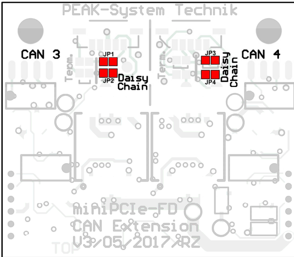
Figure 8: Position of the solder fields on the top side of the expansion card of the four-channel card (IPEH-004047) for the activation of the daisy chain
