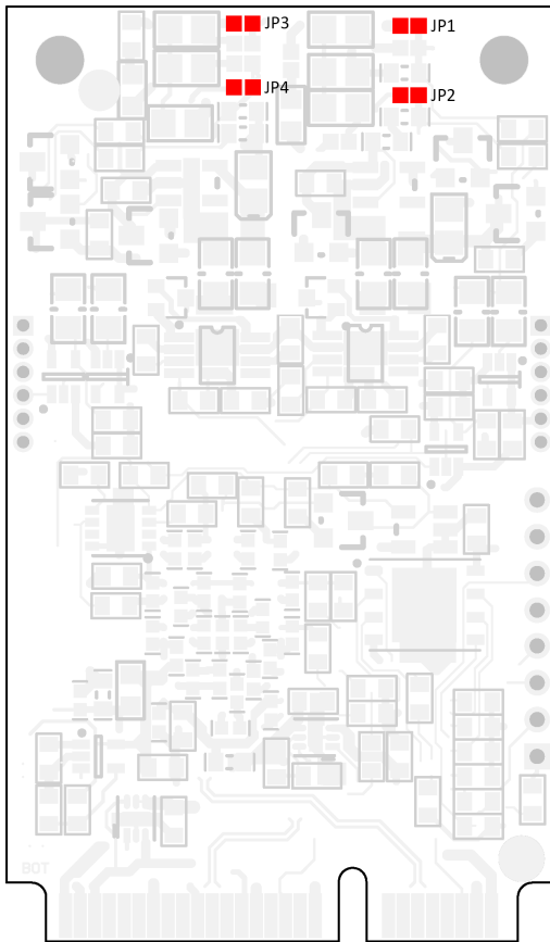
Figure 7: Position of the solder fields on the bottom side of the card (IPEH-004045/46/47) for the activation of the daisy chain
