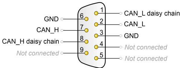
Figure 5: Pin assignment of High-speed CAN and daisy chain; male connector on the card (IPEH-004045/46/47)
