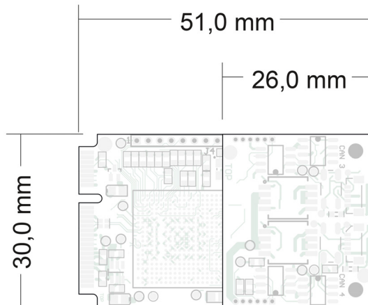
Figure 23: View onto the PCAN-miniPCIE FD Four Channel (IPEH-004047). Due to its height (approx 12 mm), the four-channel version does not comply to the form factor PCI Express Mini.
