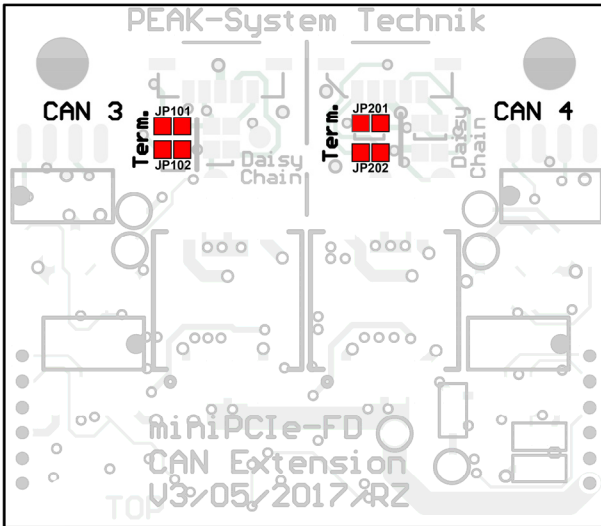
Figure 10: Position of the solder fields on the top side of the expansion card of the four-channel card ( IPEH-004047 ) for the activation of the internal termination
