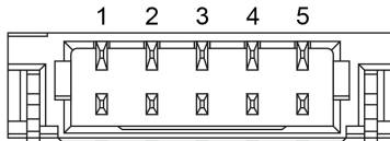
Figure 6: Front view of a CAN connector (SUR) on the PCAN-miniPCIE FD card (CAN 1 to 4)
