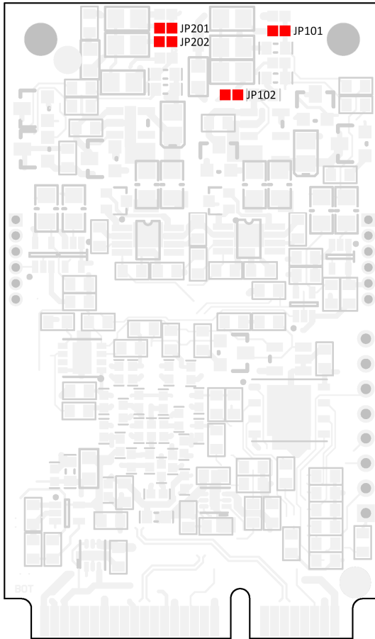
Figure 9: Position of the solder fields on the bottom side of the card (IPEH-004045/46/47) for the activation of the internal termination
