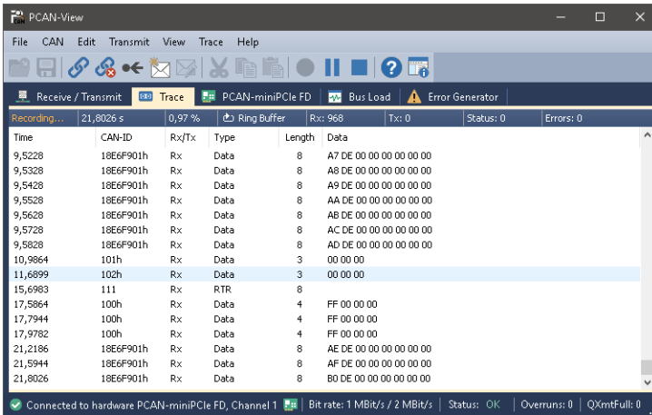
Figure 16: Trace tab
