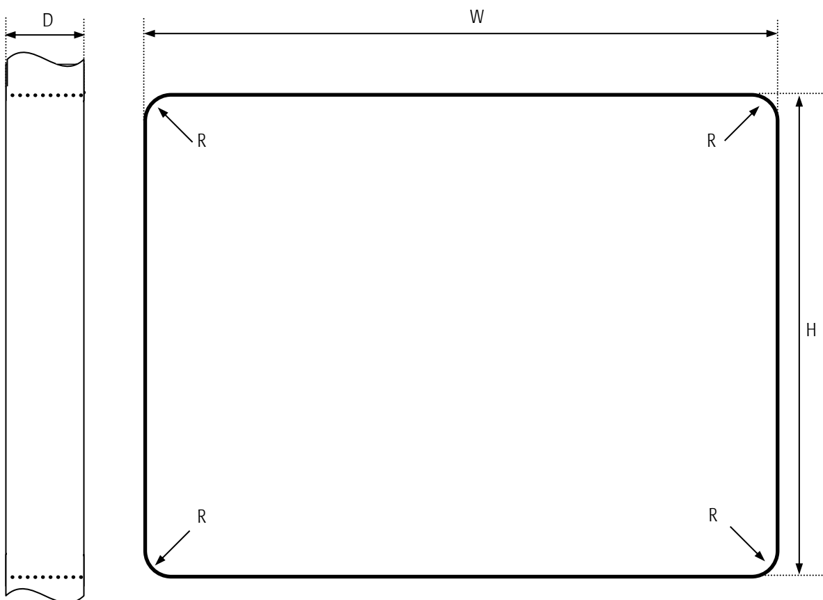
Fig. 7 Required Cut out HBxxxPU8yyy-zZZZ
