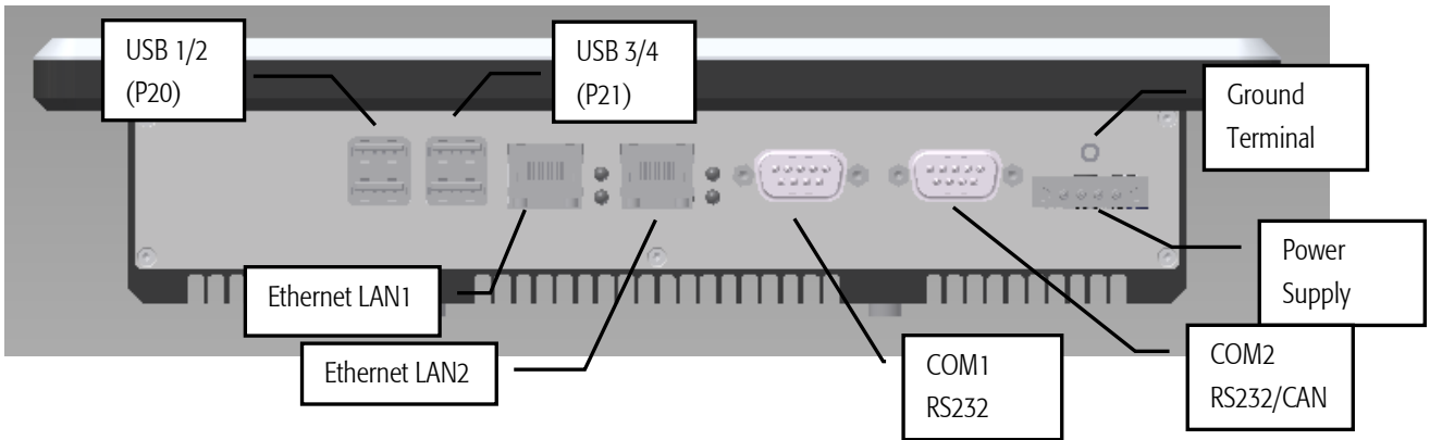
Fig. 3 HVxxxPU8yyy-zZZZ (Front)
