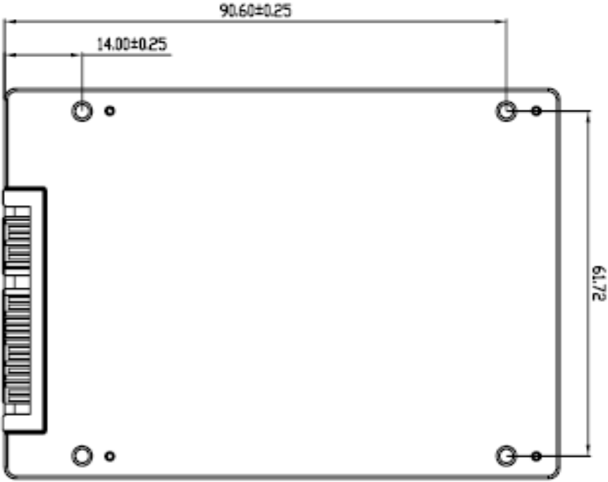
Figure 2-1. 2.5” SSD Dimensions
